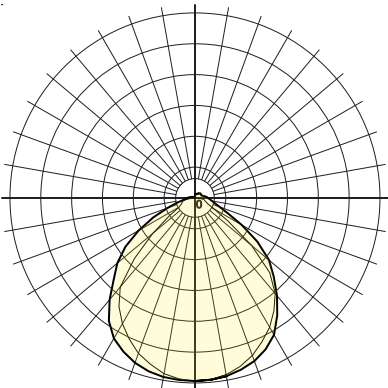
Nominal polar curve 4x14W, 1200, K19, 4000K
