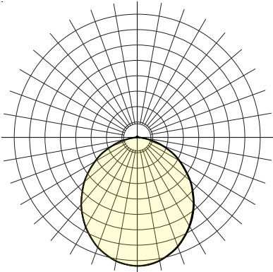
Nominal polar curve 2x14W, 1200x300, 4000K
