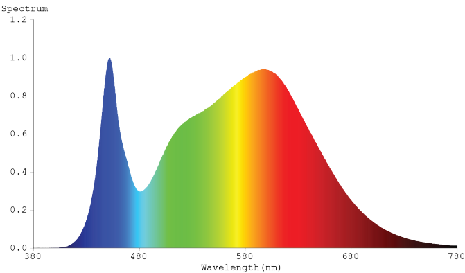
840 Spectral curve, information sourced from LED manufacturer.
