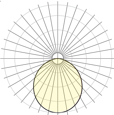
Nominal polar curve SMD8-35W-E, 4000K
