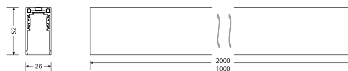
LX26-SUS1000/SUS2000
